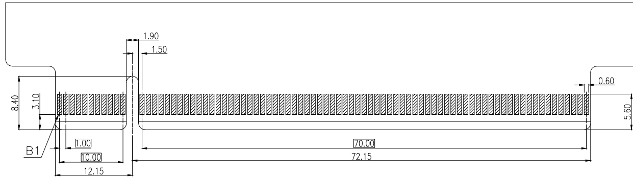
I/O PANEL DIRECTION SECONDARY (SOLDER) SIDE
