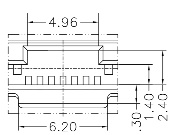
VIEW 0 SCALE 2:1
