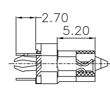
SECT B-B
