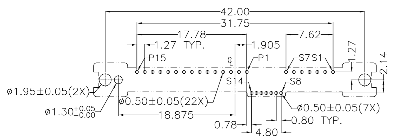
PCB LAYOUT(T=1.60mm) COMPONENT SIDE
