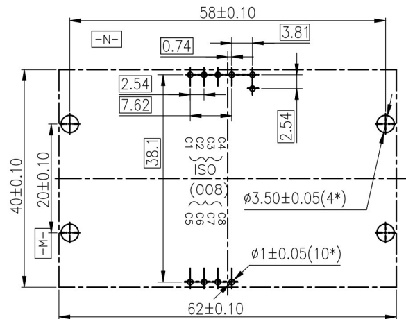
PCB Layout (Recommend)
