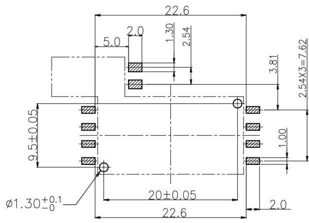
PCB Layout (component side view) Recommend(Tolerance:±0.10)
