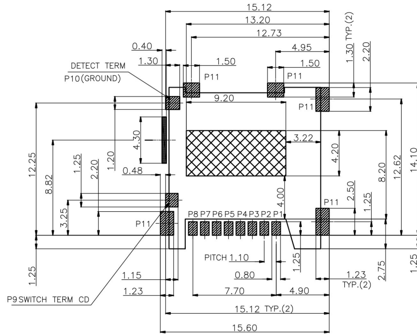
PCB PATTERN LAYOUT (GENERAL TOLERANCE:±0.05)
